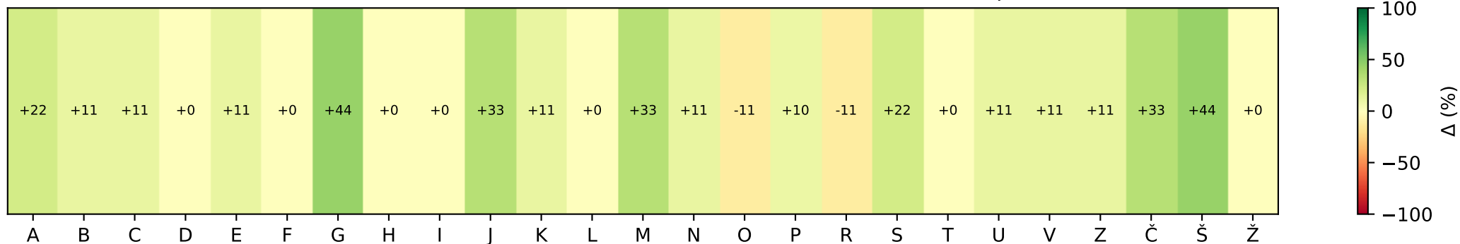
\Delta_k = \text{Točnost}_E - \text{Točnost}_D (Model E: Strokes vs Model D: Bitmaps)
